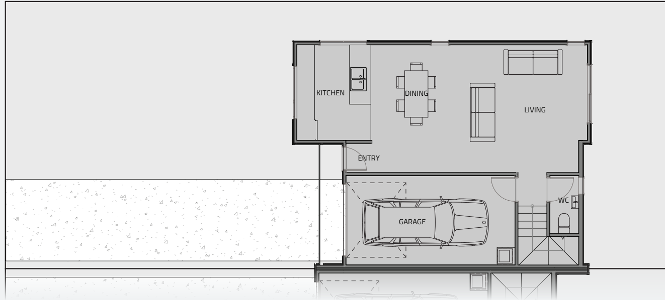
Ground Floor
